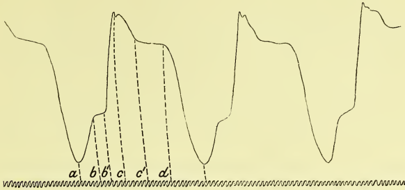
FIG. 35 1 . TRACING FROM HEART OF CAT, OBTAINED BY PLACING A LIGHT LEVER ON THE VENTRICLE, THE CHEST HAVING BEEN OPENED. THE TUNING-FORK CURVE MARKS 50 VIBRATIONS PER SEC.
